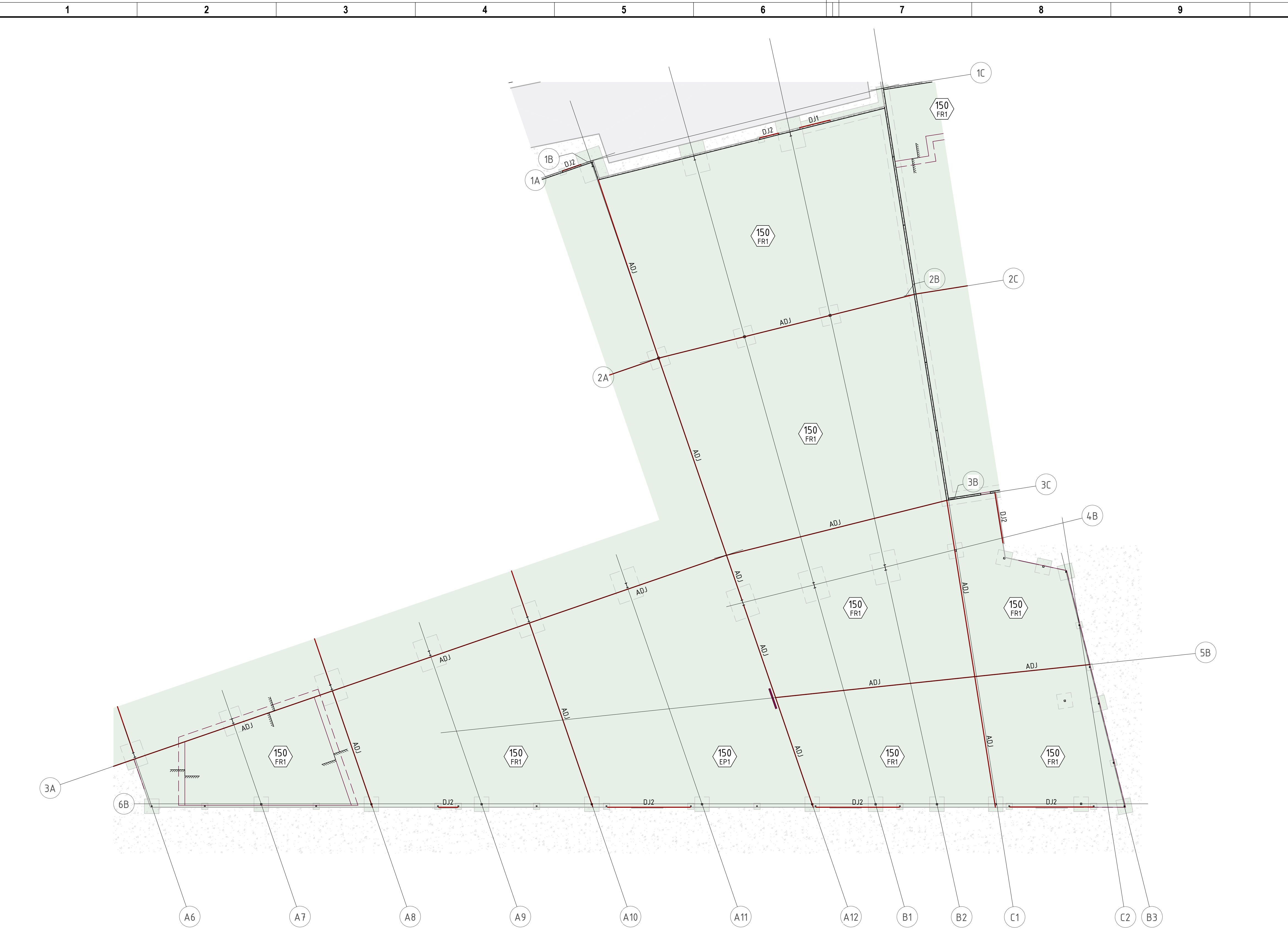
INTERNAL SLAB ON GROUND PLAN - PART 2 SCALE 1 : 200
